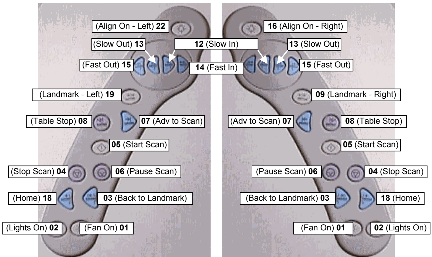
BUTTONS/DISPLAY CODES (MR/i, CV/i) ILLUSTRATION 2-1
